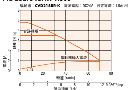
PKP262FD15AW-H50S
