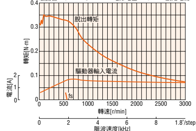
PKP244D23A2/ PKP244D23B2
