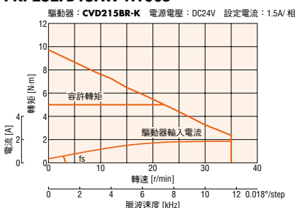
PKP262FD15AW-H100S
