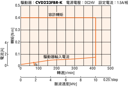
PKP243D15A2-SG18-R2FL
