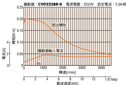
PKP233D23A/PKP233D23B
