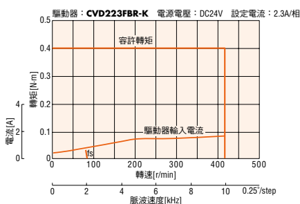
PKP243D23A2-SG18-R2FL
